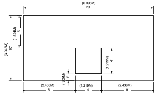
PLAN VIEW
