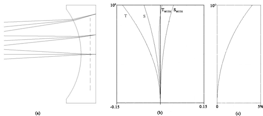
Figure 11.22. (a) Basic field flattener showing image shift from original image plane, (b) astigmatic field curves with ( T_{WITH} and S_{WITH} ) and without ( T and S ) the field flattener, and (c) distortion caused by field flattener.
