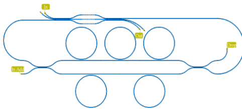
Fig. 1. Representation of an integrated optical circuit. Almost impossible to simulate with electromagnetic simulators, this circuit takes just few seconds for several hundreds of wavelenghts to be analysed with a model based simulator.
