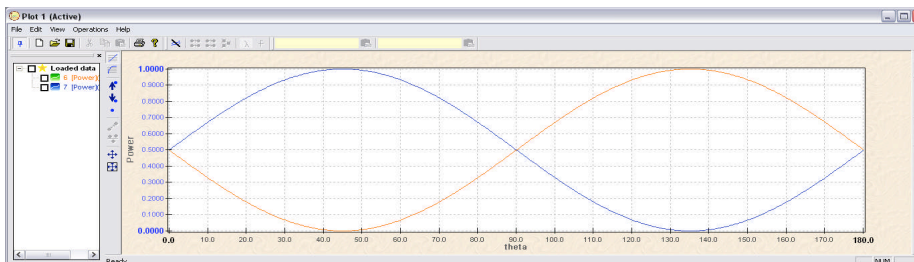
Fig. 4. Output power at the left side (red) and the right side (blue). Since the polarizer placed on the right side is oriented 45^\circ clockwise with respect to the one on the left, there is a maximum transmitted power at an imposed field rotation of 45^\circ (clockwise) passing from left to right and a minimum entering from the opposite side.
