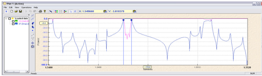
Fig. 2. Simulated spectral response of the circuits represented in fig. 1.
