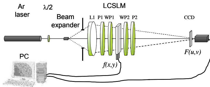
Figure 1. Convergent Diffractometer. WP1 and WP2 are wave plates and P1 and P2 are polarizers. LCSLM is the liquid crystal spatial modulator.
