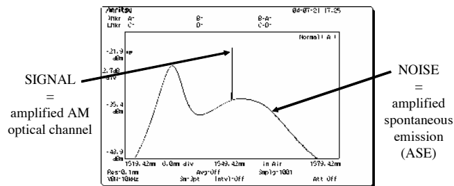
Fig.0 : typical EDFA's output spectrum
