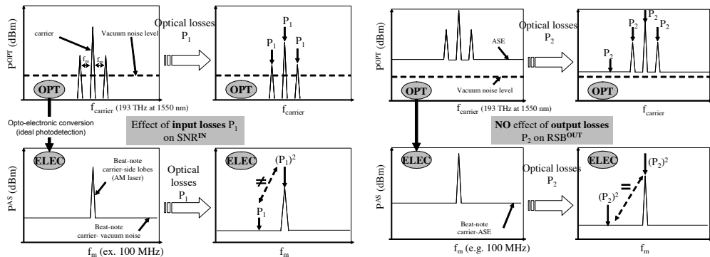
Fig. 2 . Effect of input (left) and output (right) losses on SNR (OPT stands for OPTICAL domain, ELEC for ELECTrical domain)
