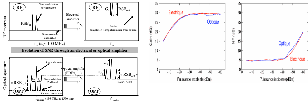
Fig. 3 .Definition of SNR and NF through an electrical or optical amplifier (left) : application to the case of an EDFA for both optical and electrical NF measurements methods
