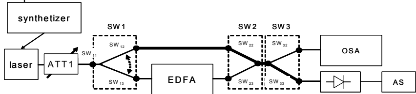
Fig. 1. Experimental set-up.
