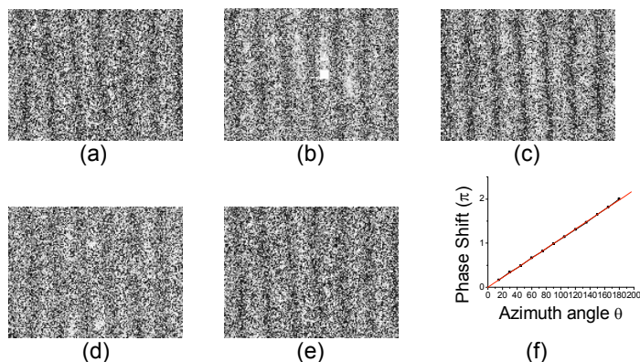
Fig.2. Interference pattern recorded onto CCD for (a) \theta = 0^\circ , (b) \theta = 45^\circ , (c) \theta = 90^\circ , (d) \theta = 135^\circ , (e) \theta = 180^\circ . (f) variation of phase shift as a function of azimuth of output polarizer.
