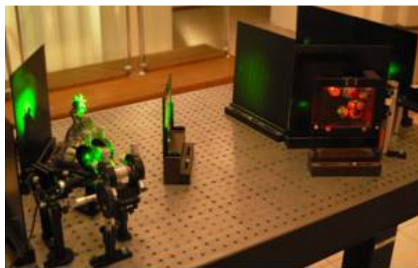
Fig.4. Model of the holographic installation
